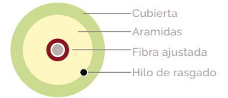
CFO 1 900
